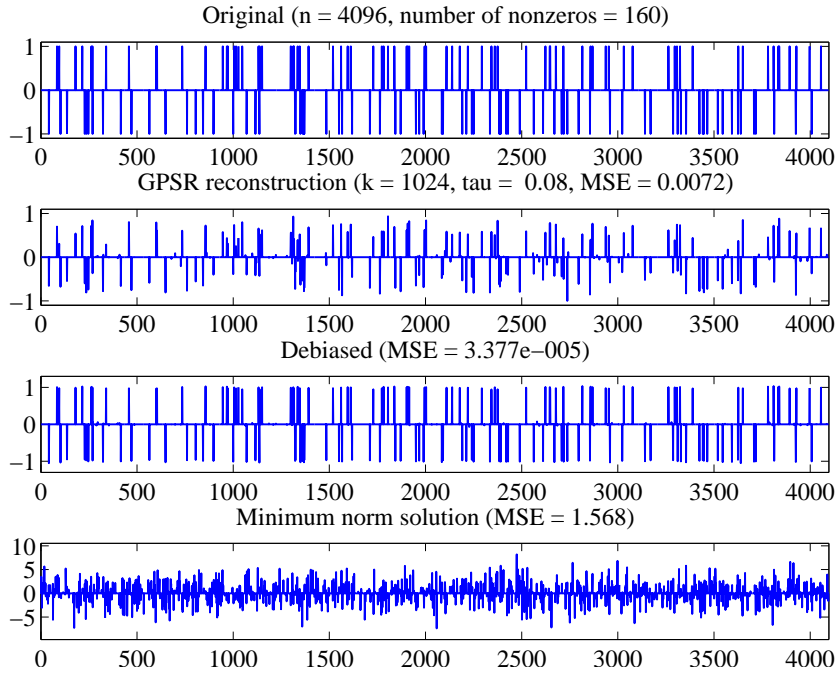
Fig. 1. From top to bottom: original signal, reconstruction via the minimization of (1) obtained by GPSR-BB, reconstruction after debiasing, the minimum norm estimate obtained using the mldivide function of MATLAB.
