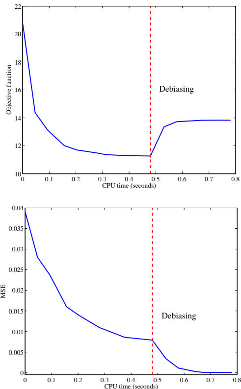
Fig. 3. Evolution of the objective function and reconstruction MSE, vs CPU time, including the debiasing phase, corresponding to the experiment illustrated in Fig. 1.
